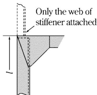
Fig. 4.8.2 Types of End Connection (Connection Type B)
