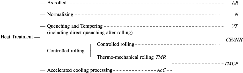
Fig. K3.1.4-1 Kind of Heat Treatment
