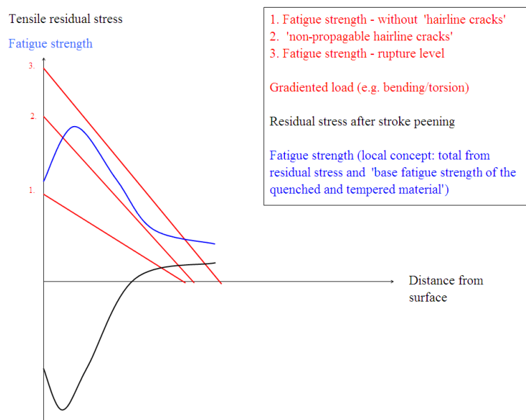
Fig. 8 Working and Residual Stresses below the Stroke-peened Surface.
