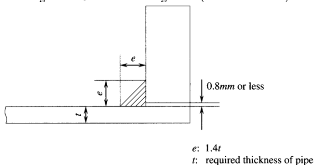
Fig. D12.4.3-2 Flange Joint (One-side Welded)
