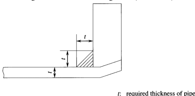
Fig. D12.4.3-1 Flange Joint (Bell-mouth)
