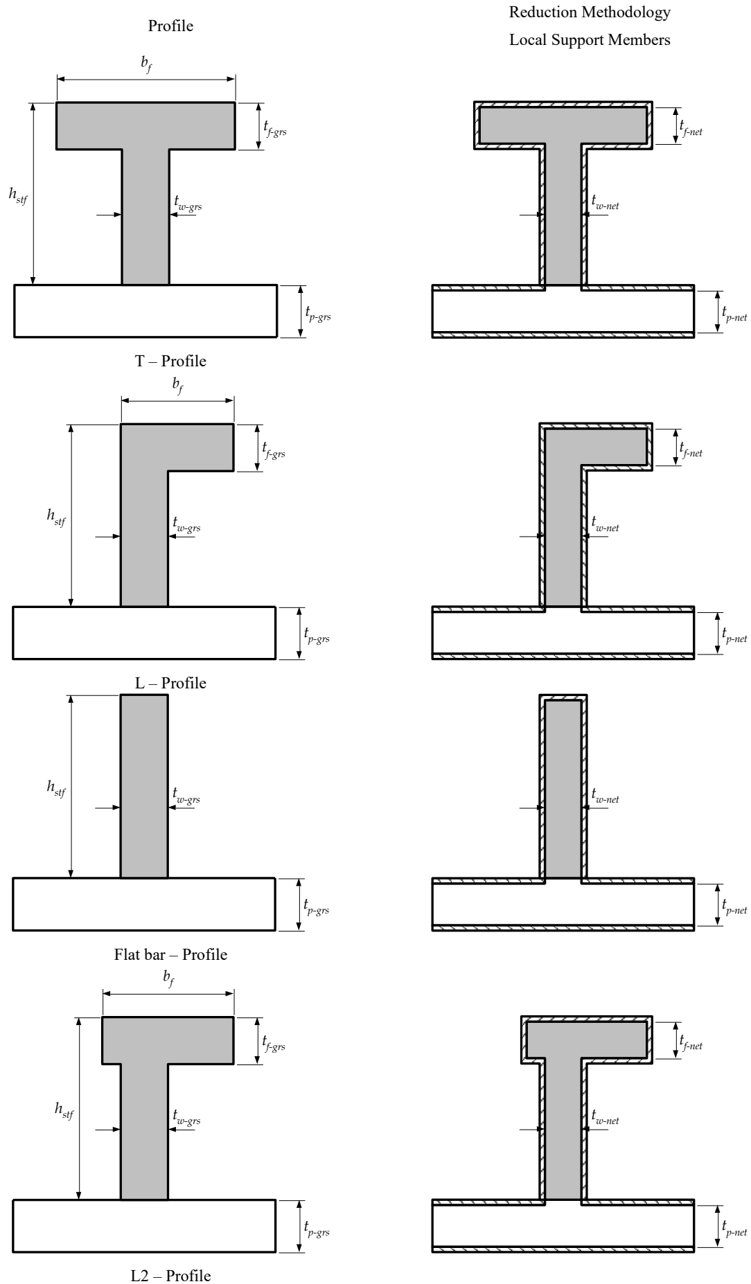
Fig. 4.2.12 Net Sectional Properties of Local Support Members
