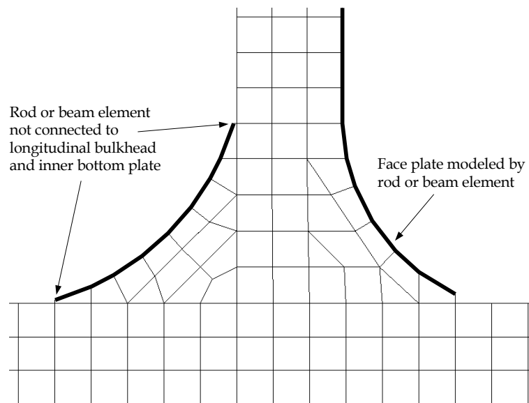
Fig. B.2.5 Typical Finite Element Mesh on Transverse Web Frame Main Bracket
