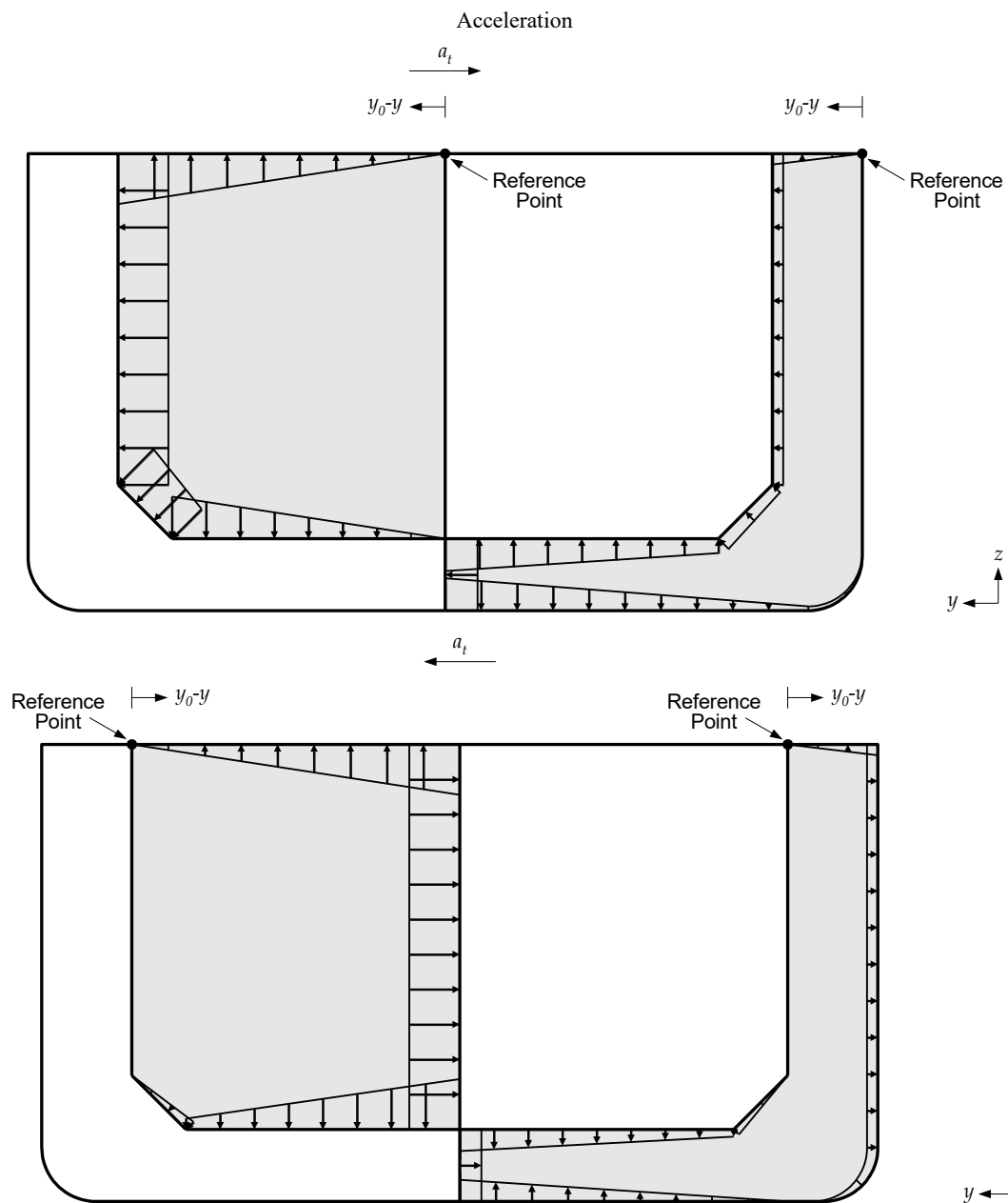
Fig. 7.6.5 Dynamic Tank Pressure in Cargo Tank (Left) and Ballast Tank (Right) due to Negative and Positive Transverse Tank
