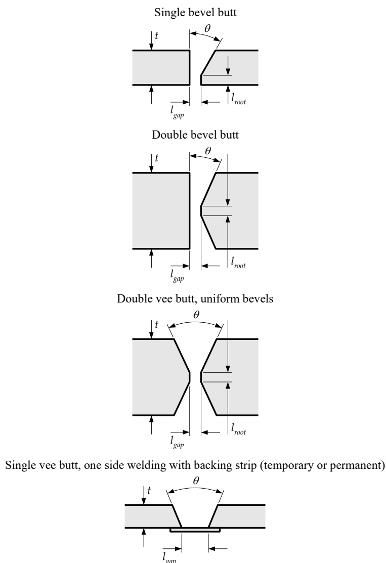
Fig. 6.5.1 Typical Butt Welds
