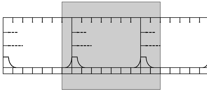
Fig. B.2.14 Extent of FE Model for Verification against Acceptance Criteria
