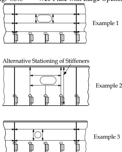
Fig. 4.3.8 Web Plate with Large Openings
