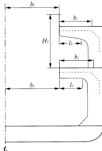
Fig. C7.3 Measurement of l_0 , b_1 , b_2 and H_2
