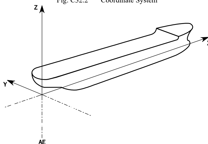
Fig. C32.2 Coordinate System
