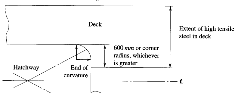
Fig. 2.3 Deck
