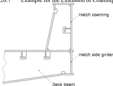
Fig. C20.7 Example for the Extension of Coaming Plates
