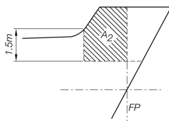
Fig. C27.3 Effective Areas for Screens, Bulwarks, etc.
