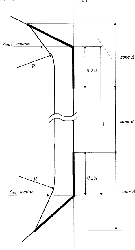
Fig. C31.3 Hold Frames and Upper and Lower Brackets
