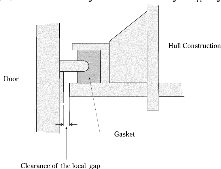
Fig C23.4.6-1 Maximum Design Clearance between Securing and Supporting Devices
