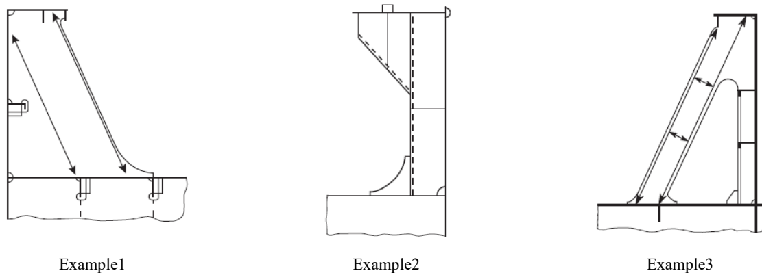
Fig. C20.6 Examples of coaming stays
