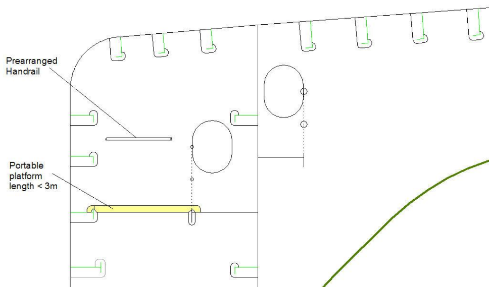
Fig. 1 Portable Platform
