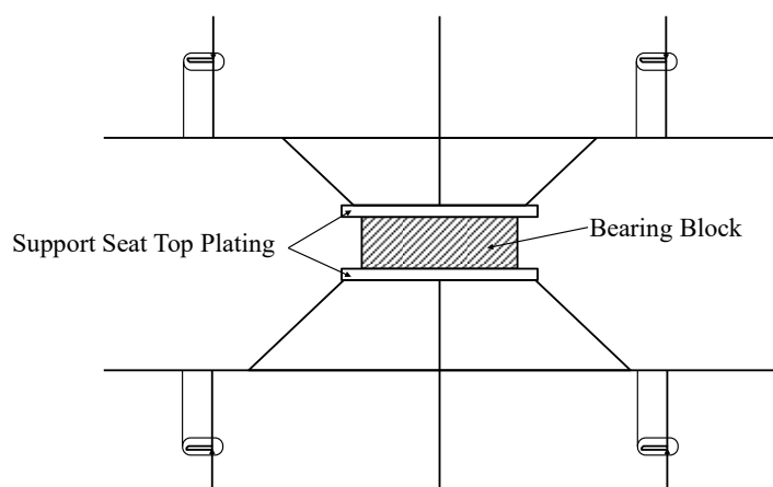
Supporting Structure Example 1
