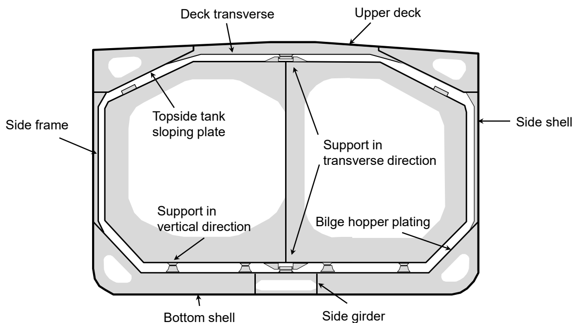
Fig. 1.2.2-2 Various Supports (Examples of Supports in Vertical, Transverse, and Longitudinal Direction )
