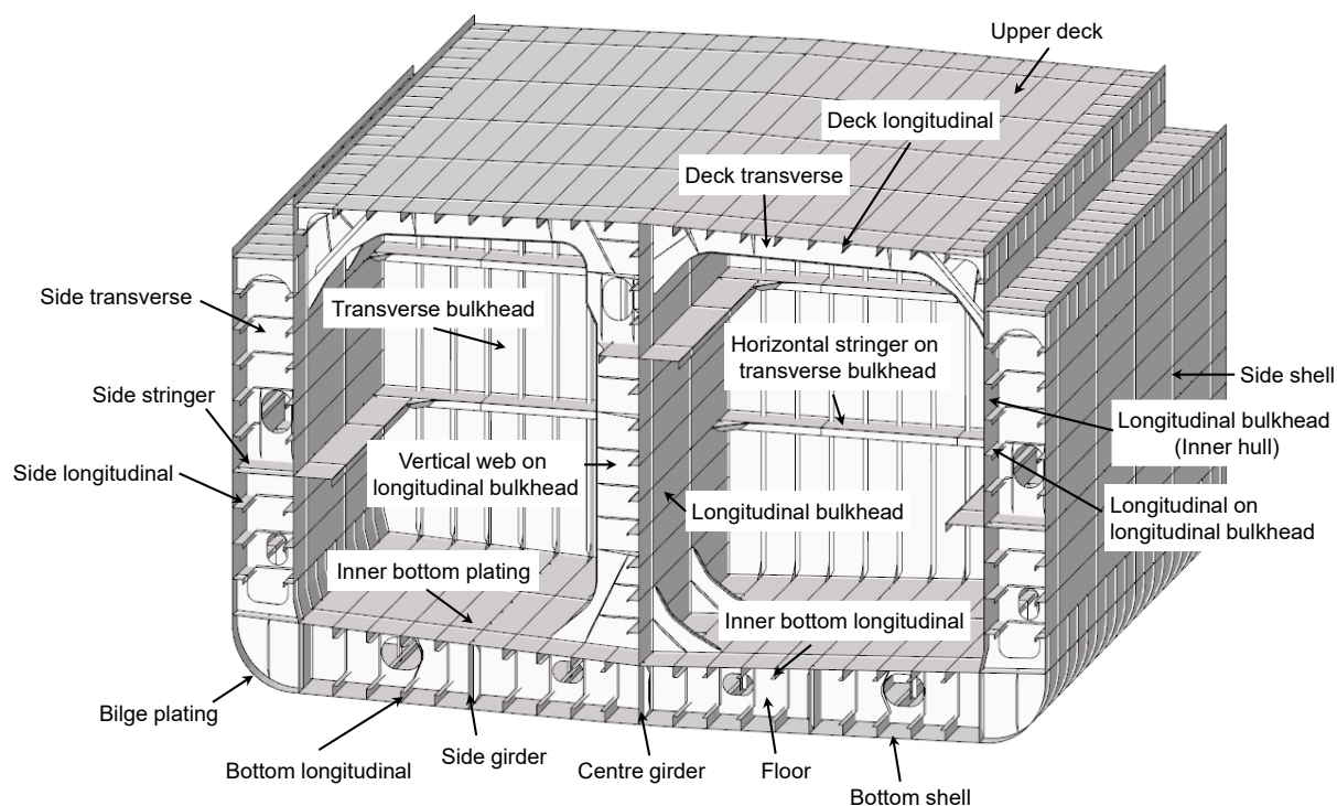
Fig. 1.2.1-2 Chemical Tankers
