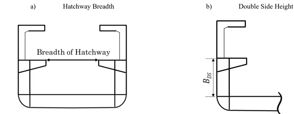
Fig. 7.3.1-1 Hatchway Breadth and Double Side Height
