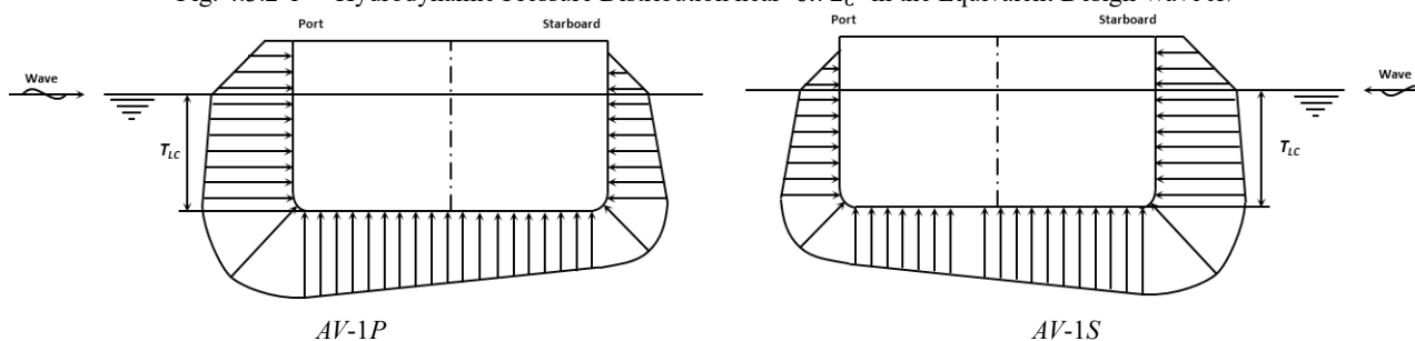
Fig. 4.3.2-1 Hydrodynamic Pressure Distribution near 0.7L_C in the Equivalent Design Wave AV
