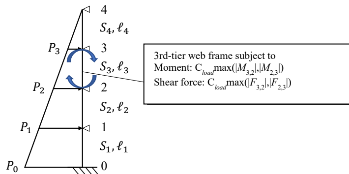
Fig. 7.2.1-2 Moment Acting on a Web Frame at Node i
