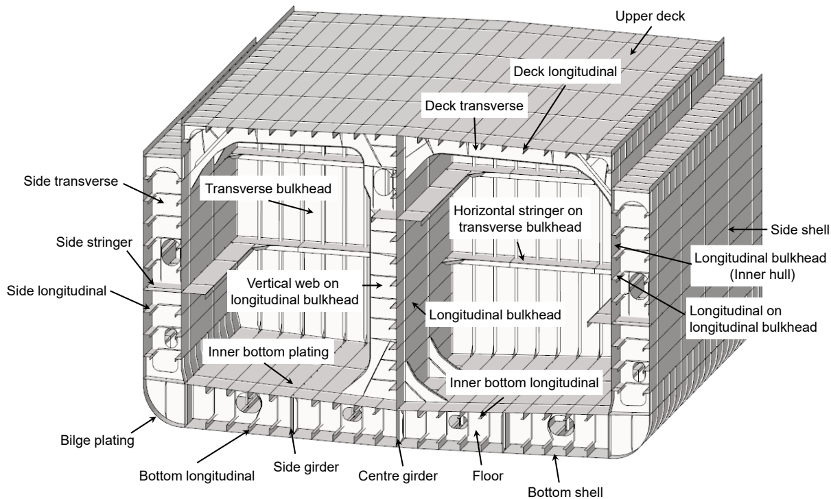
Fig. 1.2.1-2 Chemical Tankers
