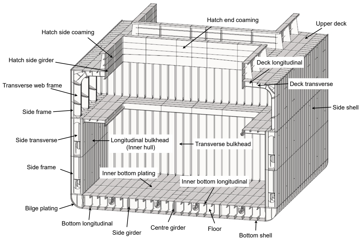
Fig. 1.2.1-2 Reefer Ships
