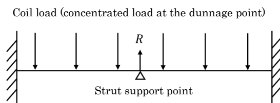
Fig. 10.1.2-2 Load Conditions Between Girders and Struts (Equidistant Load Points)
