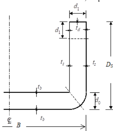
Fig. 5.5.3-1 Mean Thickness of Deck, Ship Sides, and Bottom
