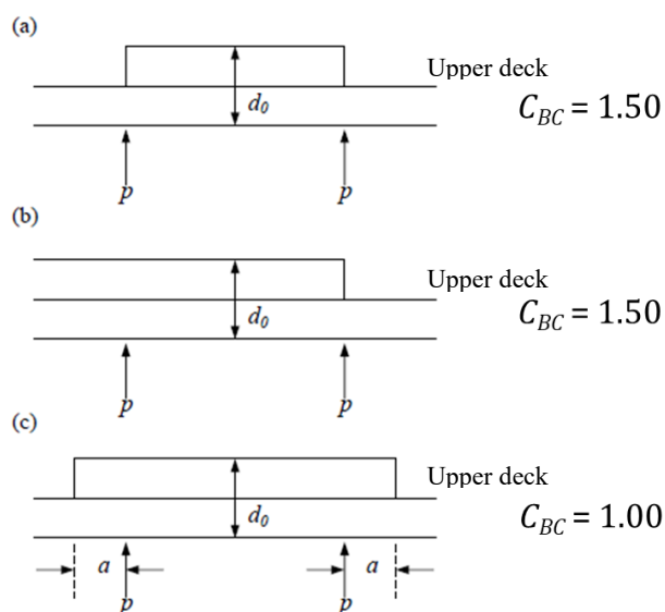
Fig. 7.2.1-1 Hatch Side Girders Supported by Pillars, etc.
