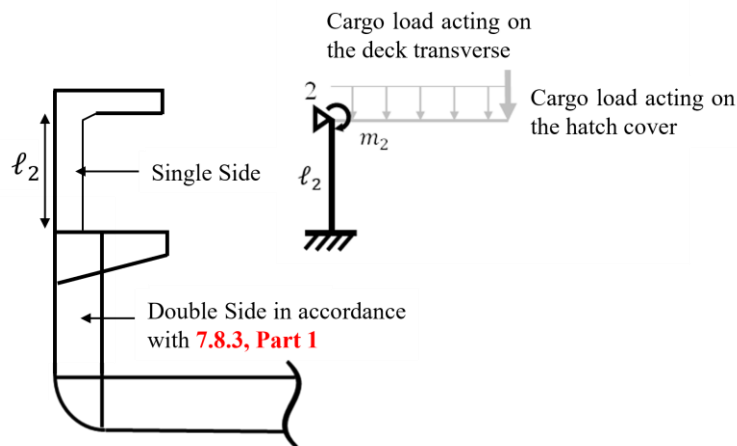
Fig. 7.2.2-1 Web Frames of Double-deck Ships with the First Layers being Double Side and the Second Layers being Single Side
