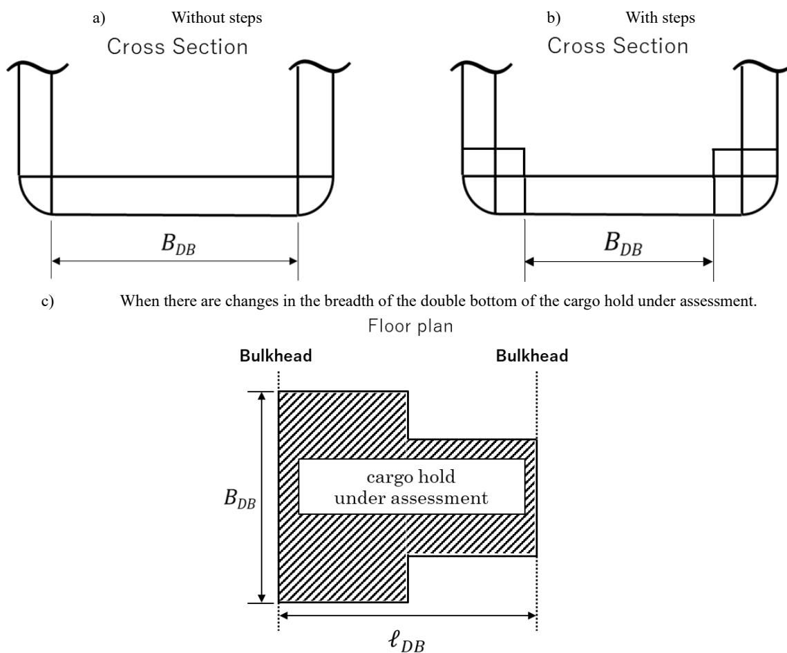
Fig. 7.2.1-1 Double Bottom Breadth
