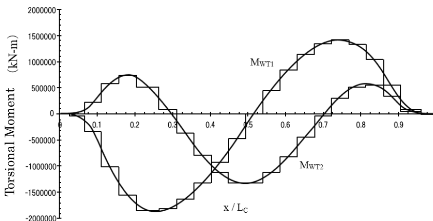
Fig. 5.5.2-3 Torsional Moments Acting on Hull Girders (Approximated Torsional Step Moment)
