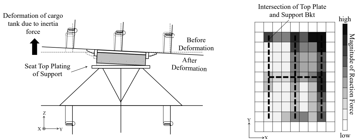
Fig. 9.4.3-1 Example of Reaction Force Distribution for Contact Surface
