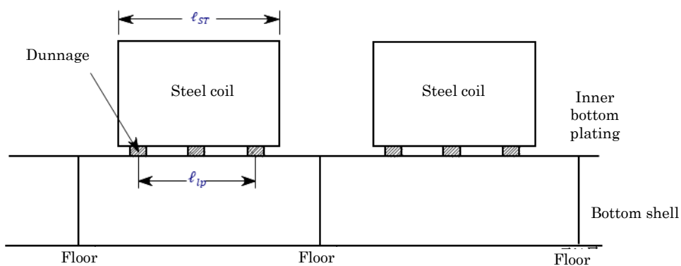
Fig. 4.4.2-3 Loading of Steel Coils on the Inner Bottom Taking into Consideration the Floor Position
