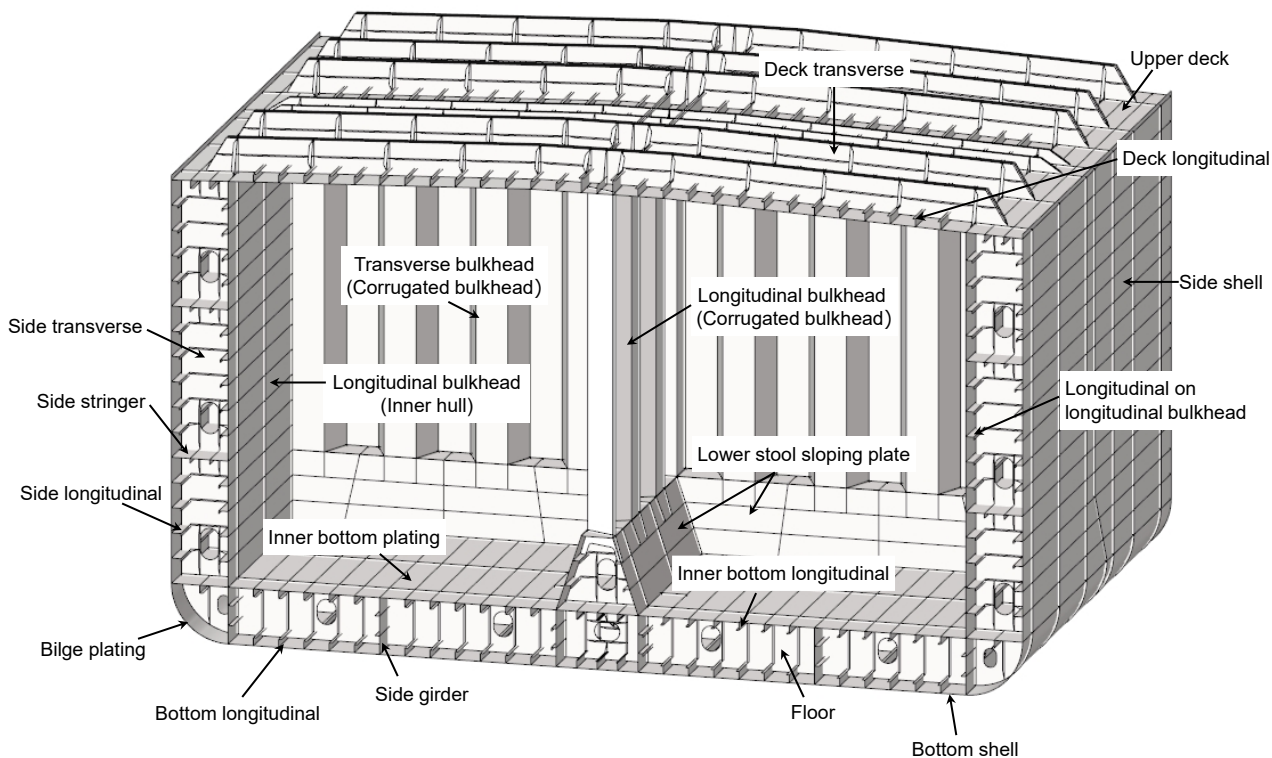
Fig. 1.2.1-2 Chemical Tankers
