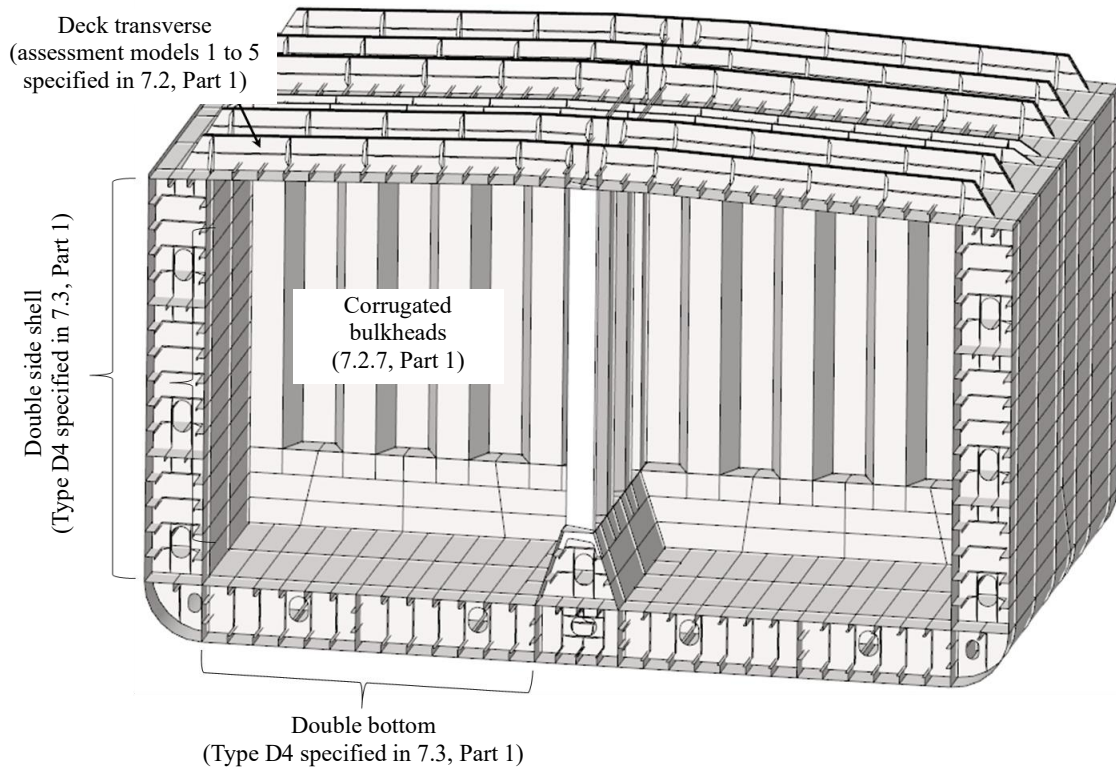
Fig. 7.1.1-2 Application Example of Chemical Tanker
