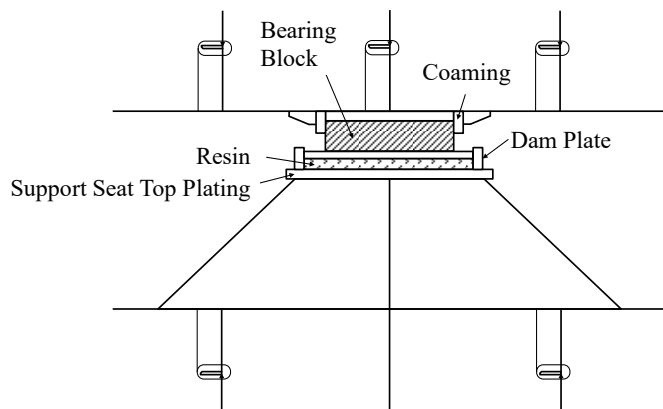
Supporting Structure Example 3
