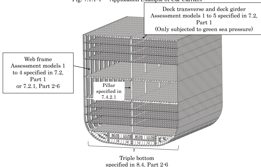
Fig. 7.1.1-1 Application Example of Car Carriers
