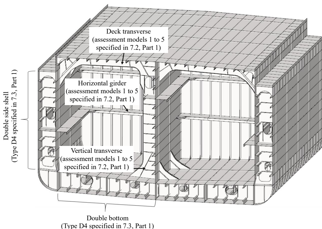
Fig. 7.1.1-1 Application Example of Oil Tanker
