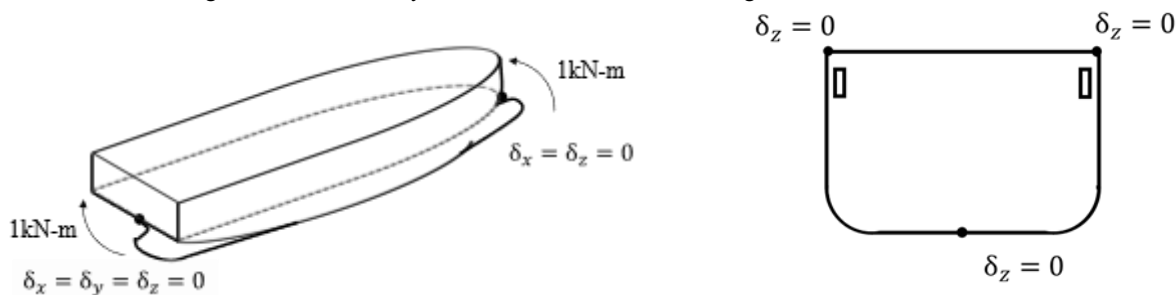
Fig. 9.4.4-3 Boundary Conditions of Horizontal Bending Moments and Load Conditions
