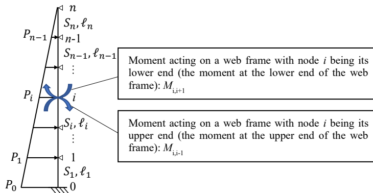
Fig. 7.2.1-2 Moment Acting on a Web Frame at Node i
