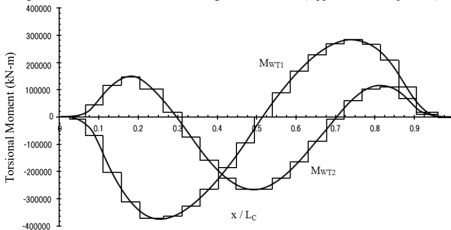
Fig. 9.4.4-4 Torsional Moments Acting on Hull Girders (Approximated Step Curve)
